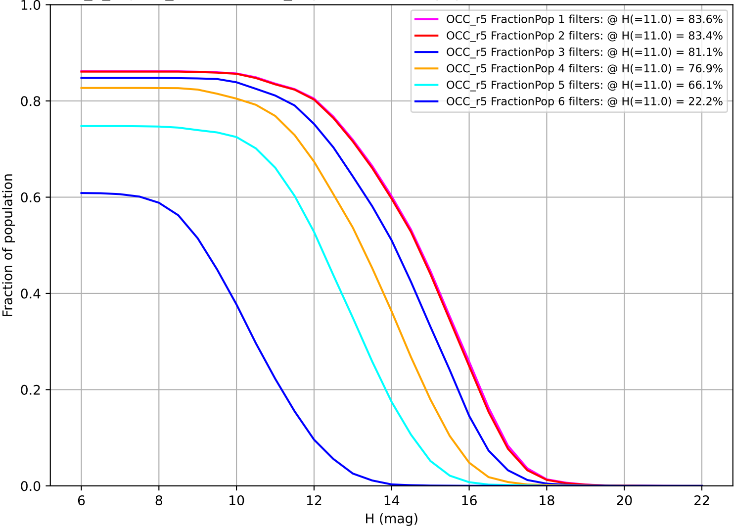
internal_u_expt27_nscale1.2v3.4_10yrs: Fraction of population with colors in X filters OCC_r5
