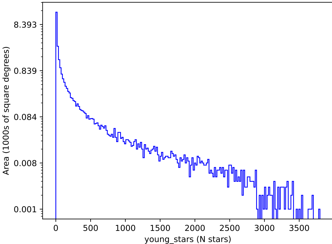
internal_u_expt27_nscales1.2v3.4_10yrs : young_stars
