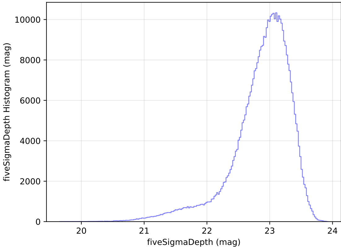
internal_u_expt27_nscale1.2v3.4_10yrs z: fiveSigmaDepth Histogram
