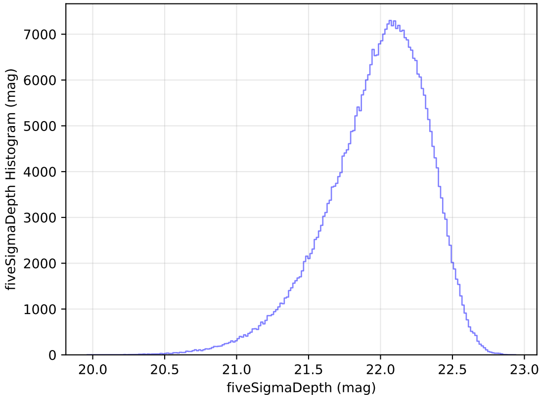
internal_u_expt27_nscale1.2v3.4_10yrs y: fiveSigmaDepth Histogram
