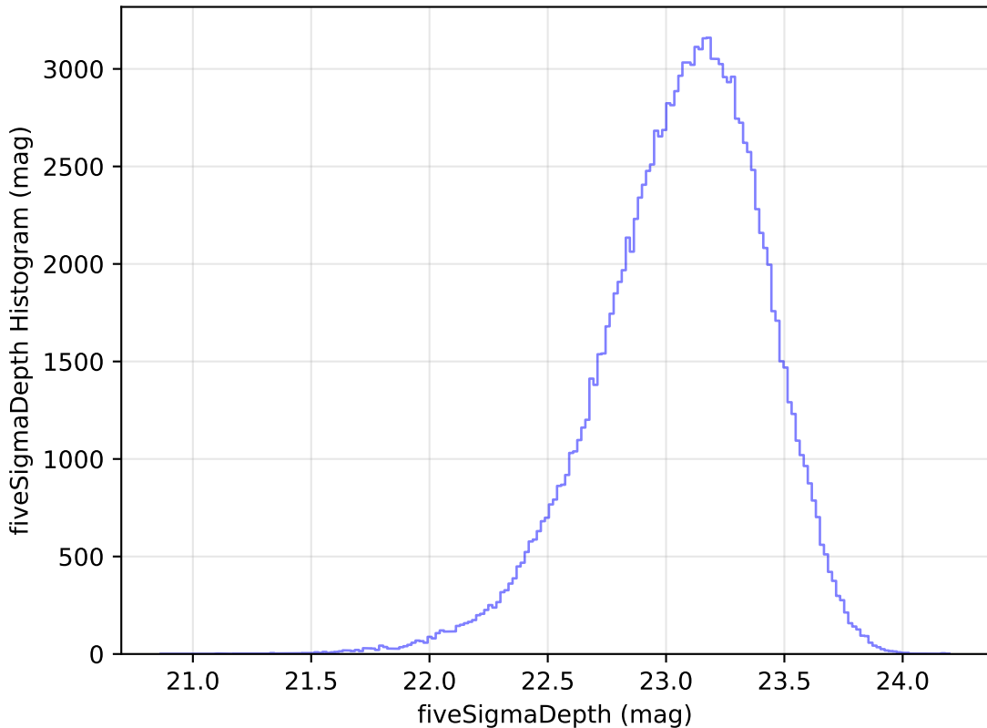
internal_u_expt27_nscale1.2v3.4_10yrs u: fiveSigmaDepth Histogram
