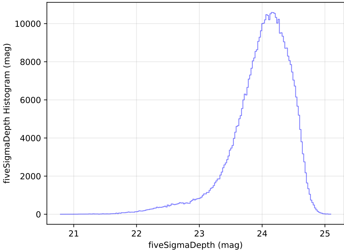
internal_u_expt27_nscale1.2v3.4_10yrs r: fiveSigmaDepth Histogram
