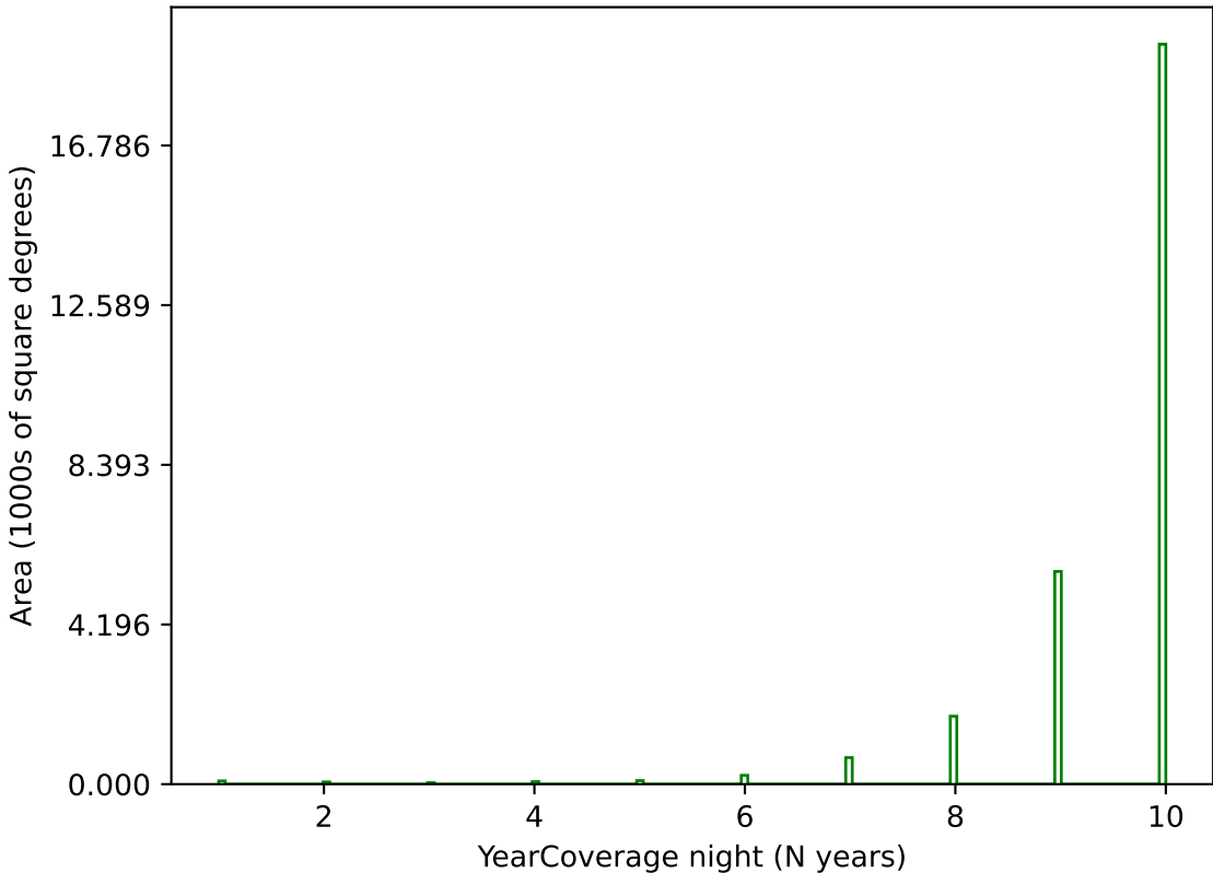
internal_u_expt27_nscale1.2v3.4_10yrs g band: YearCoverage night
