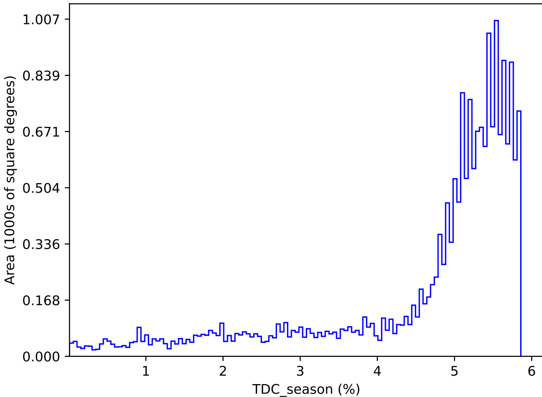
internal_u_expt27_nscale1.2v3.4_10yrs : TDC_season
