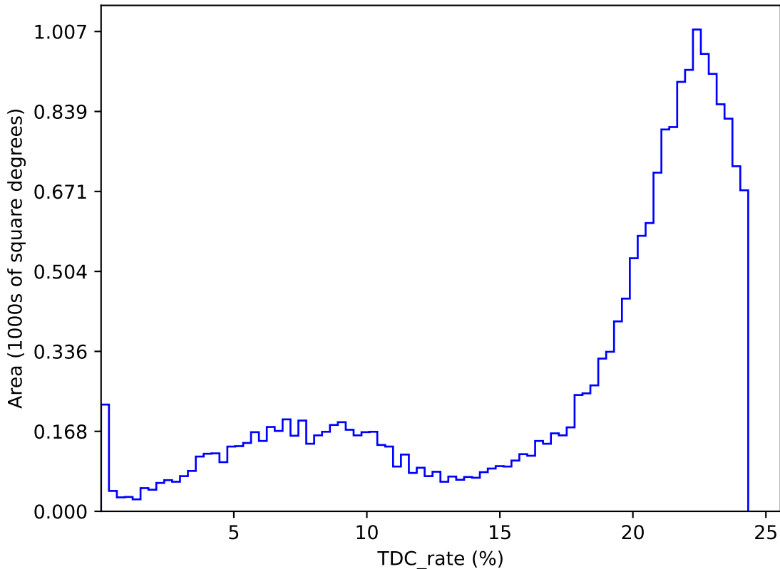
internal_u_expt27_nscale1.2v3.4_10yrs : TDC_rate
