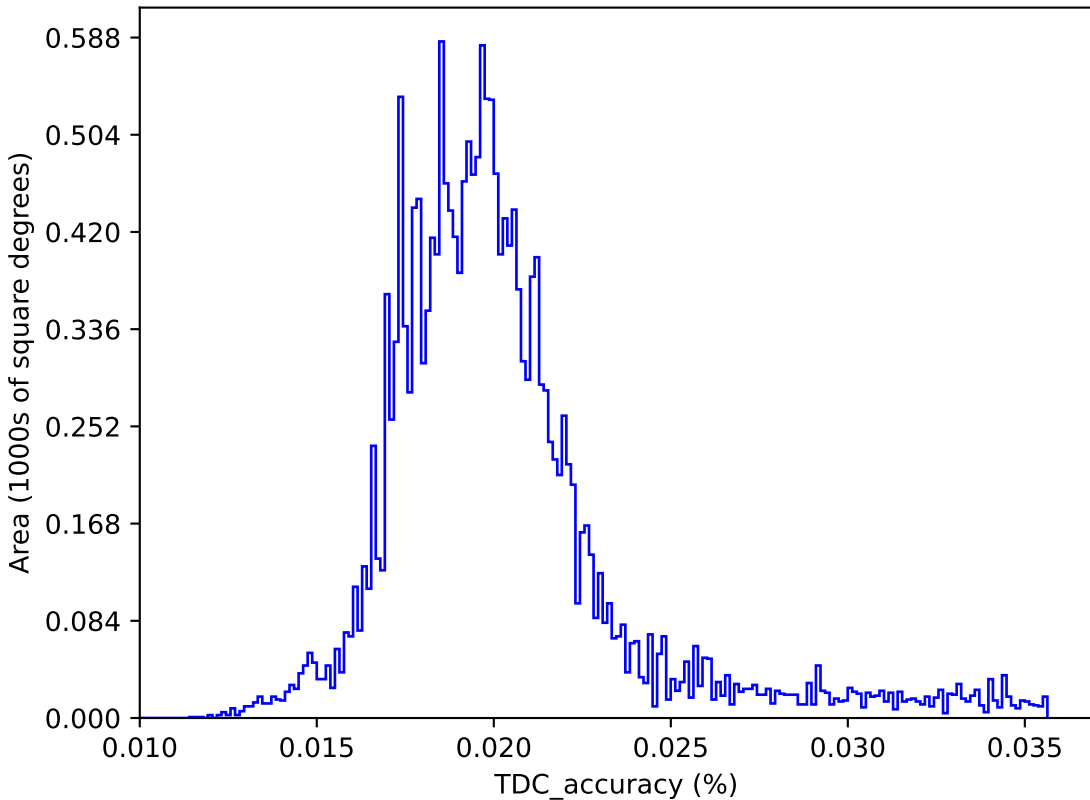
internal_u_expt27_nscale1.2v3.4_10yrs : TDC_accuracy
