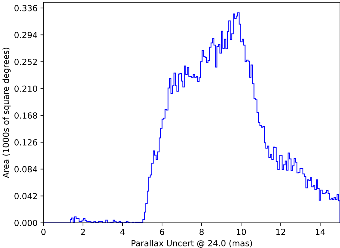
internal_u_expt27_nscale1.2v3.4_10yrs : Parallax Uncert @ 24.0
