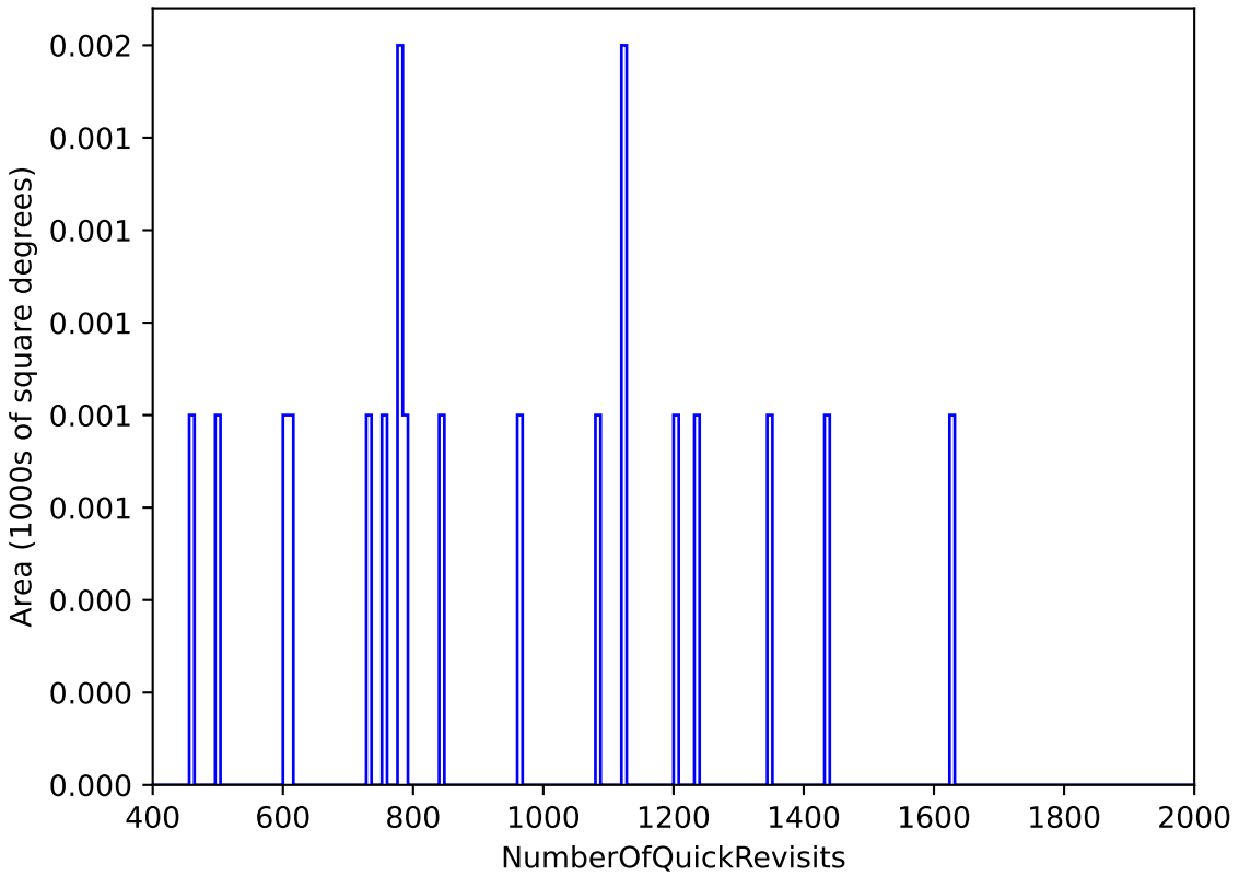
internal_u_expt27_nscale1.2v3.4_10yrs : NumberOfQuickRevisits
