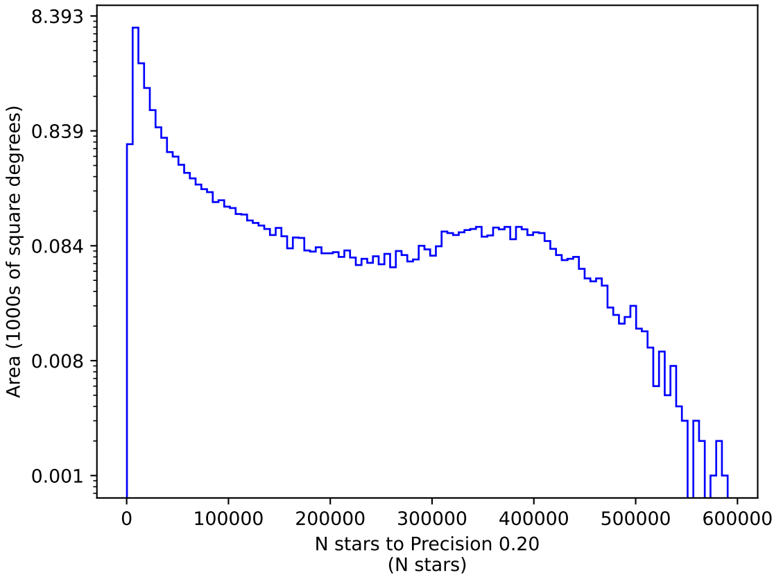
internal_u_expt27_nscale1.2v3.4_10yrs y: N stars to Precision 0.20
