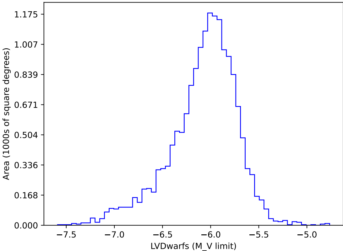
internal_u_expt27_nscale1.2v3.4_10yrs gi: LVDwarfs
