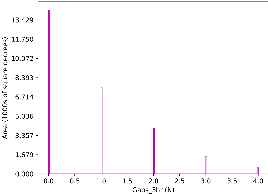
internal_u_expt27_nscale1.2v3.4_10yrs z band: Gaps_3hr
