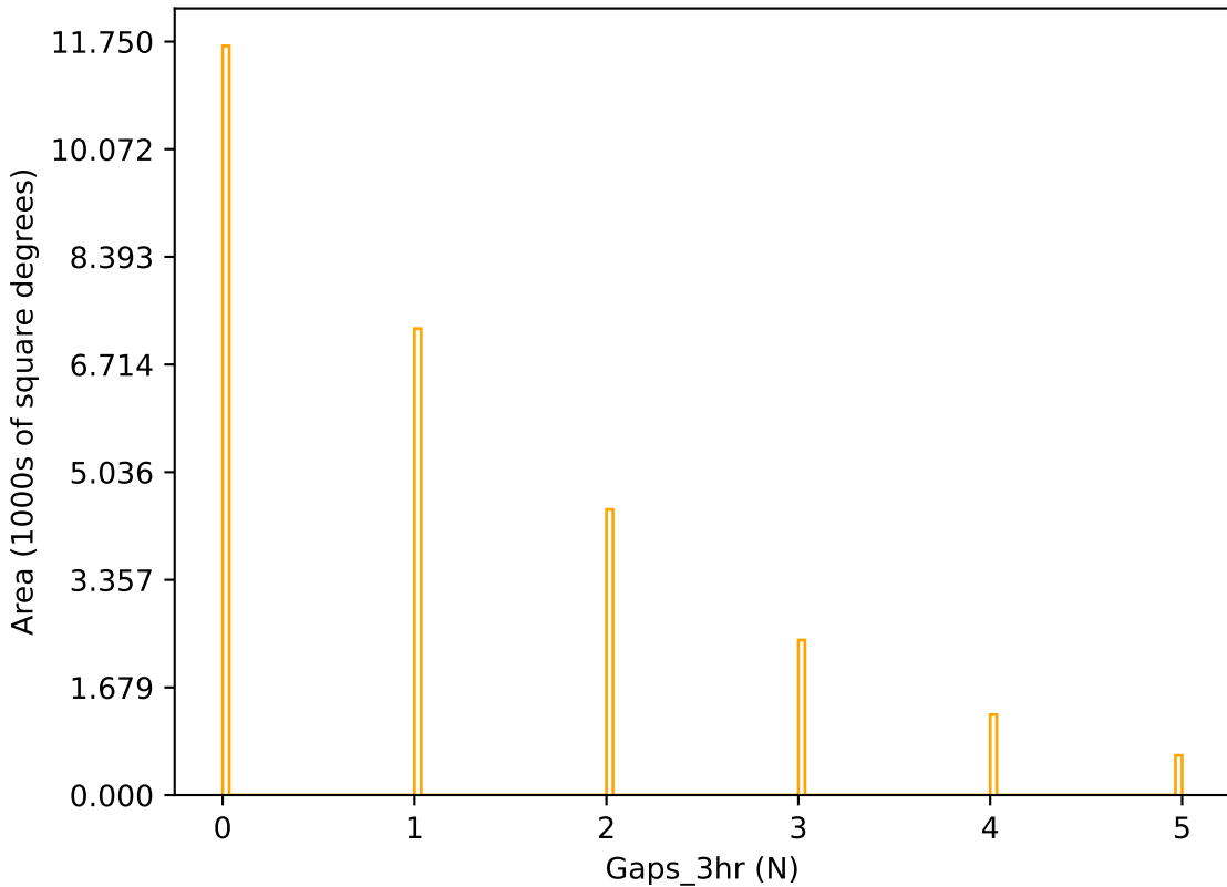
internal_u_expt27_nscale1.2v3.4_10yrs r band: Gaps_3hr
