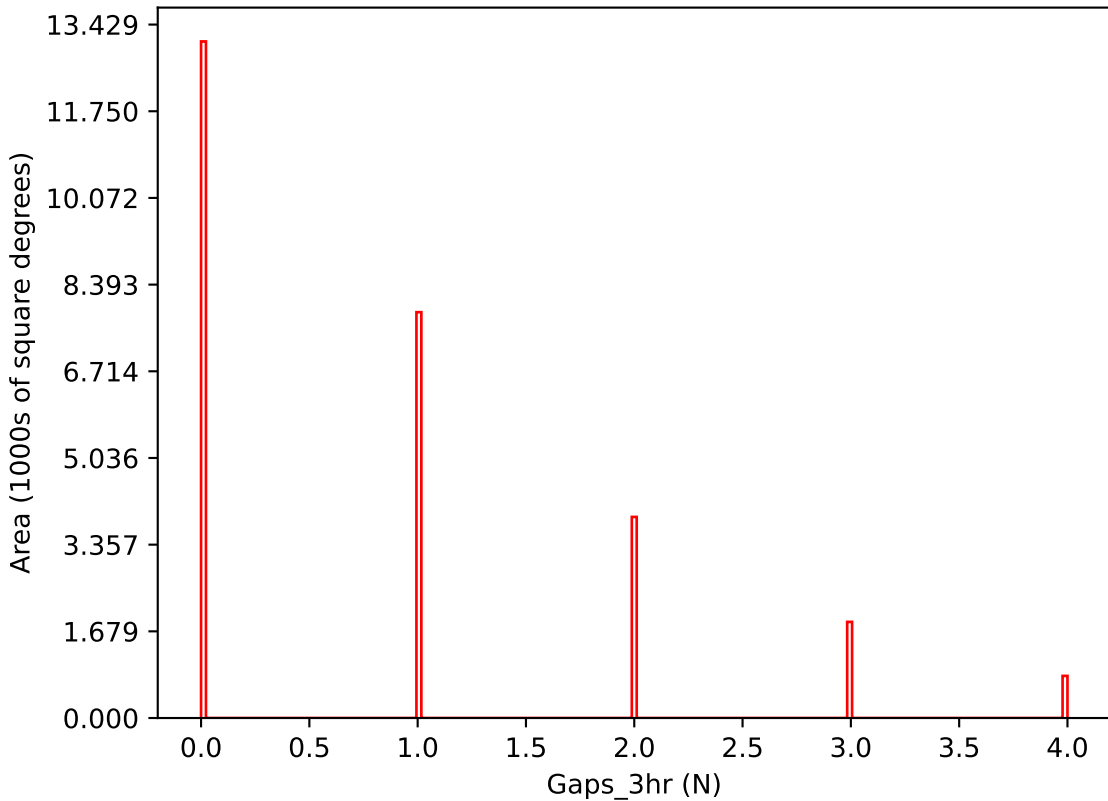
internal_u_expt27_nscale1.2v3.4_10yrs i band: Gaps_3hr
