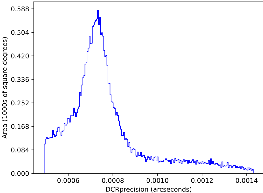
internal_u_expt27_nscale1.2v3.4_10yrs : DCRprecision
