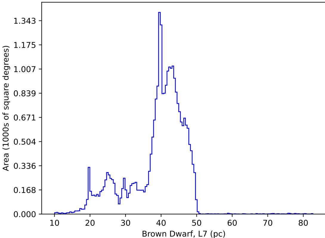
internal_u_expt27_nscale1.2v3.4_10yrs : Brown Dwarf, L7
