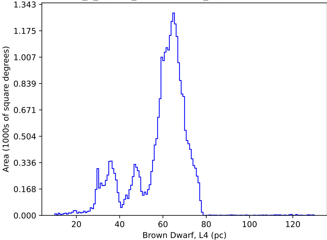
internal_u_expt27_nscale1.2v3.4_10yrs : Brown Dwarf, L4
