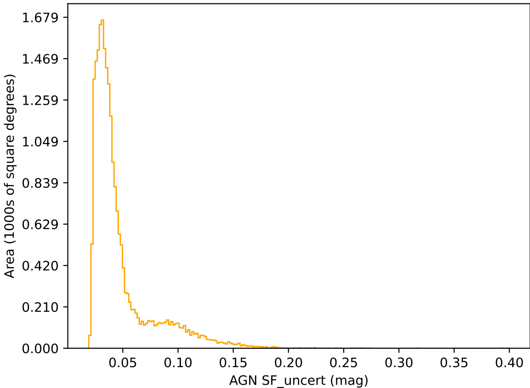
internal_u_expt27_nscale1.2v3.4_10yrs r band: AGN SF_uncert
