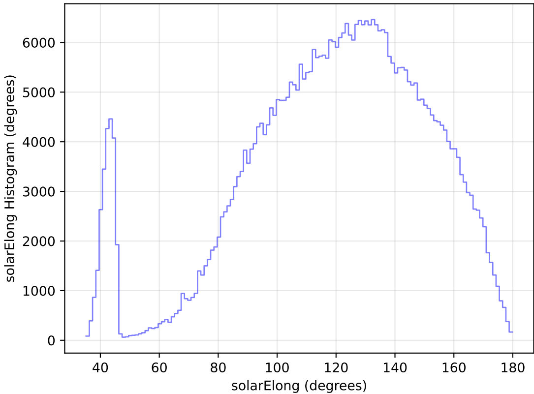
internal_u_expt27_nscale1.2v3.4_10yrs WFD z band: solarElong Histogram
