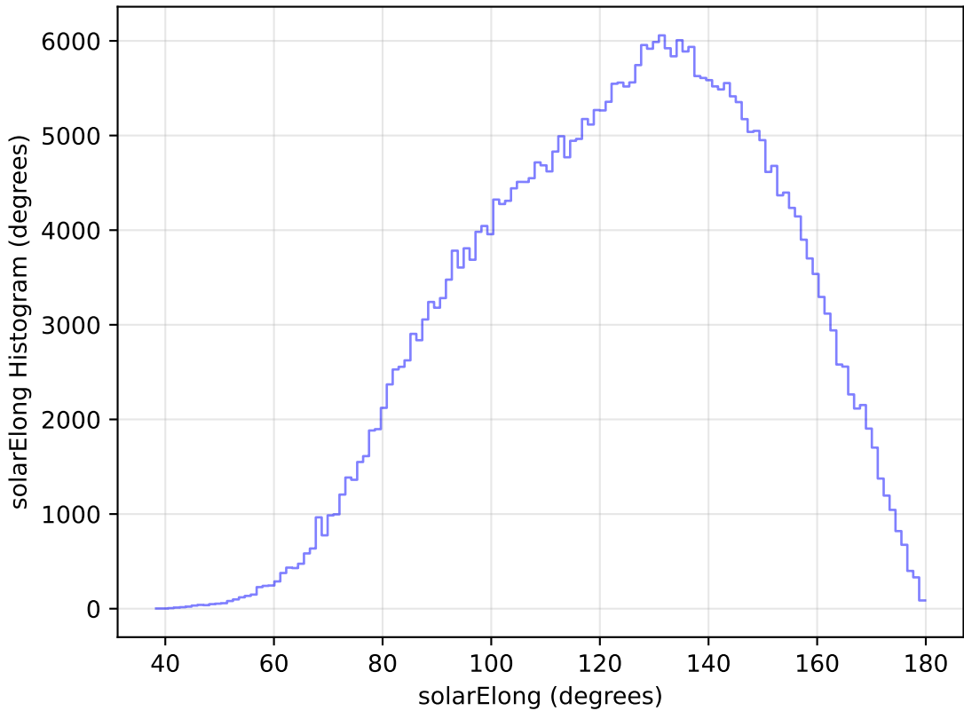
internal_u_expt27_nscale1.2v3.4_10yrs WFD y band: solarElong Histogram
