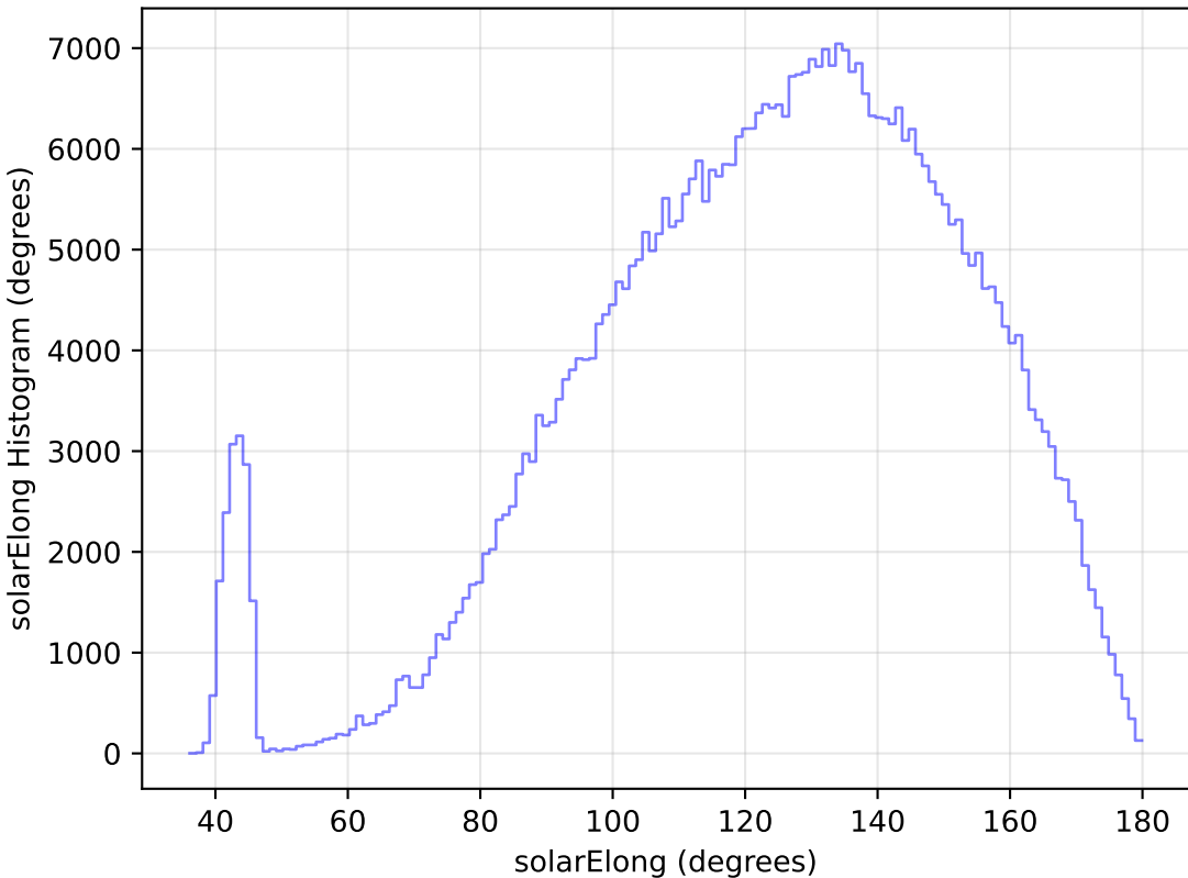
internal_u_expt27_nscale1.2v3.4_10yrs WFD r band: solarElong Histogram
