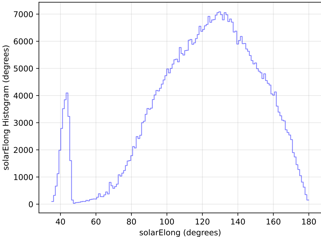
internal_u_expt27_nscale1.2v3.4_10yrs WFD i band: solarElong Histogram
