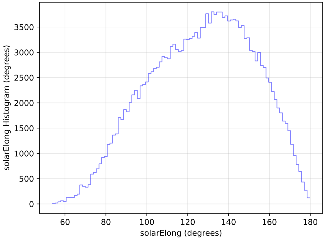
internal_u_expt27_nscale1.2v3.4_10yrs WFD g band: solarElong Histogram
