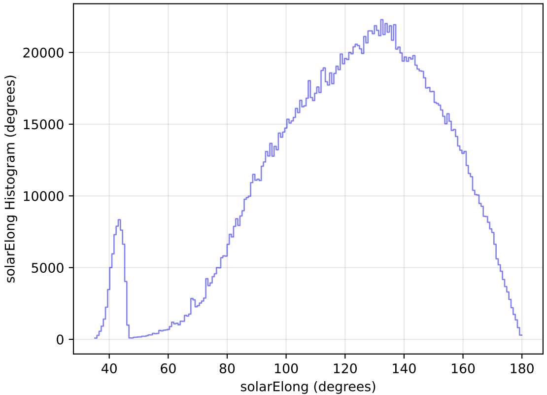
internal_u_expt27_nscale1.2v3.4_10yrs WFD all bands: solarElong Histogram
