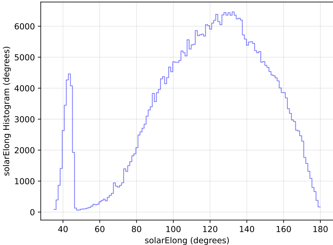
internal_u_expt27_nscale1.2v3.4_10yrs All sky z band: solarElong Histogram
