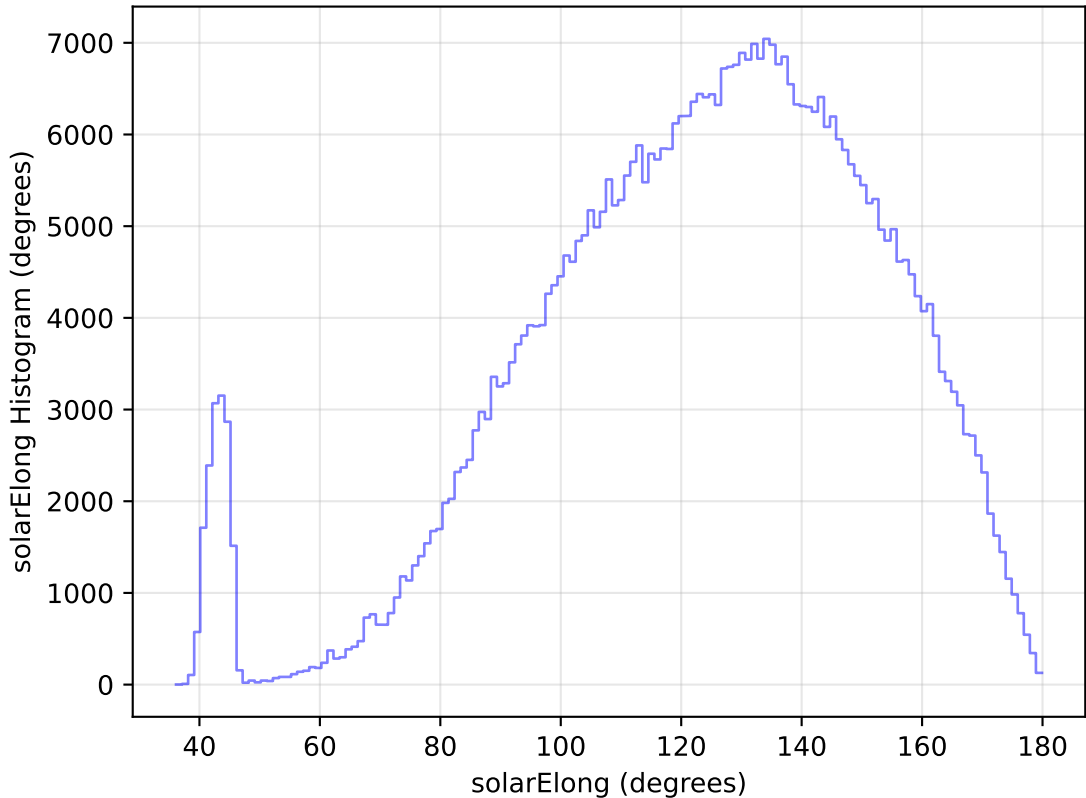
internal_u_expt27_nscale1.2v3.4_10yrs All sky r band: solarElong Histogram
