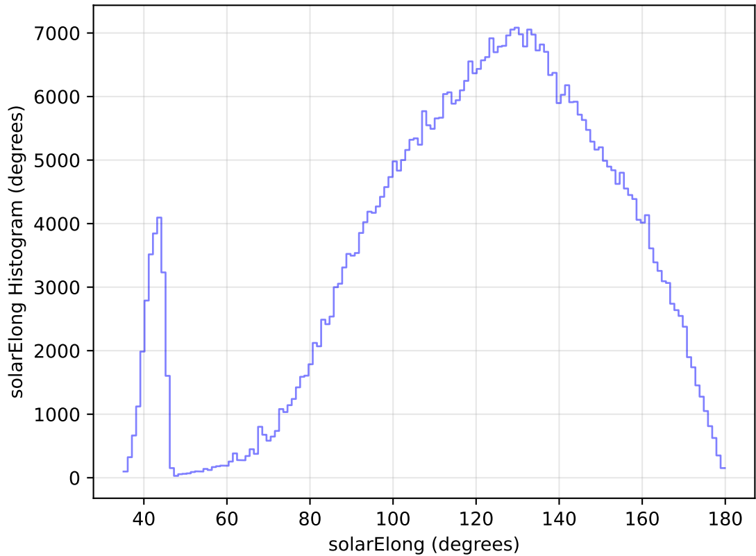
internal_u_expt27_nscale1.2v3.4_10yrs All sky i band: solarElong Histogram
