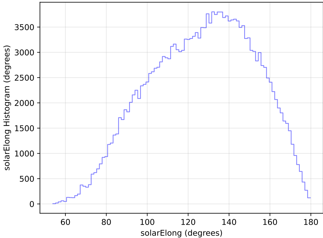
internal_u_expt27_nscale1.2v3.4_10yrs All sky g band: solarElong Histogram
