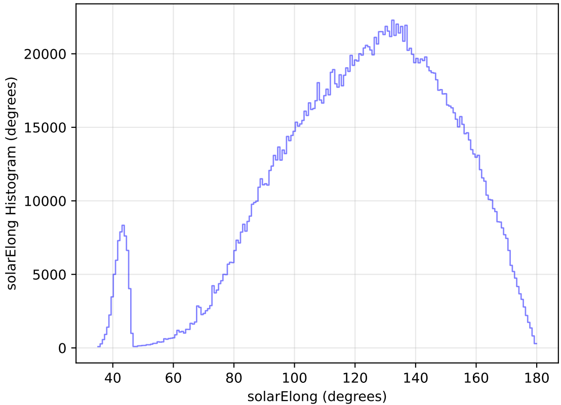
internal_u_expt27_nscale1.2v3.4_10yrs All sky all bands: solarElong Histogram
