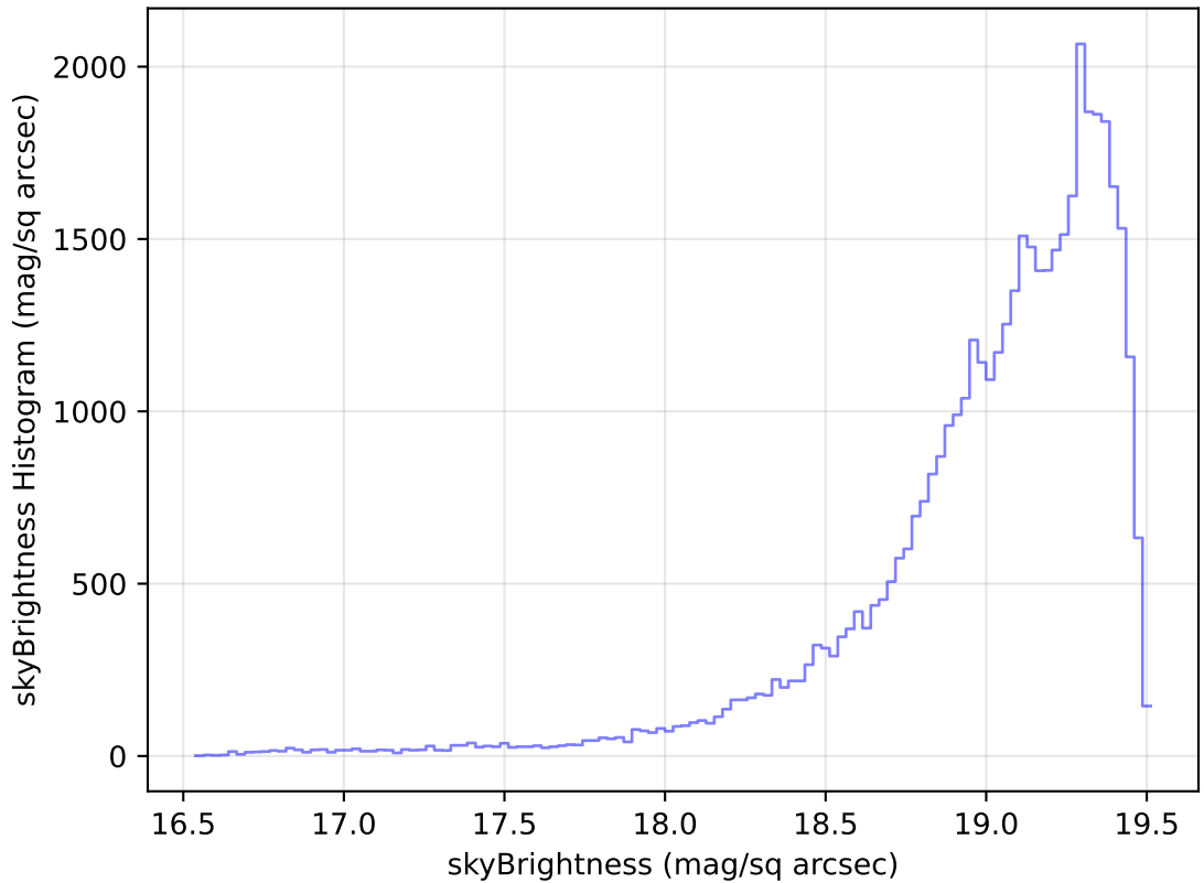
internal_u_expt27_nscale1.2v3.4_10yrs Yr 1 z band: skyBrightness Histogram
