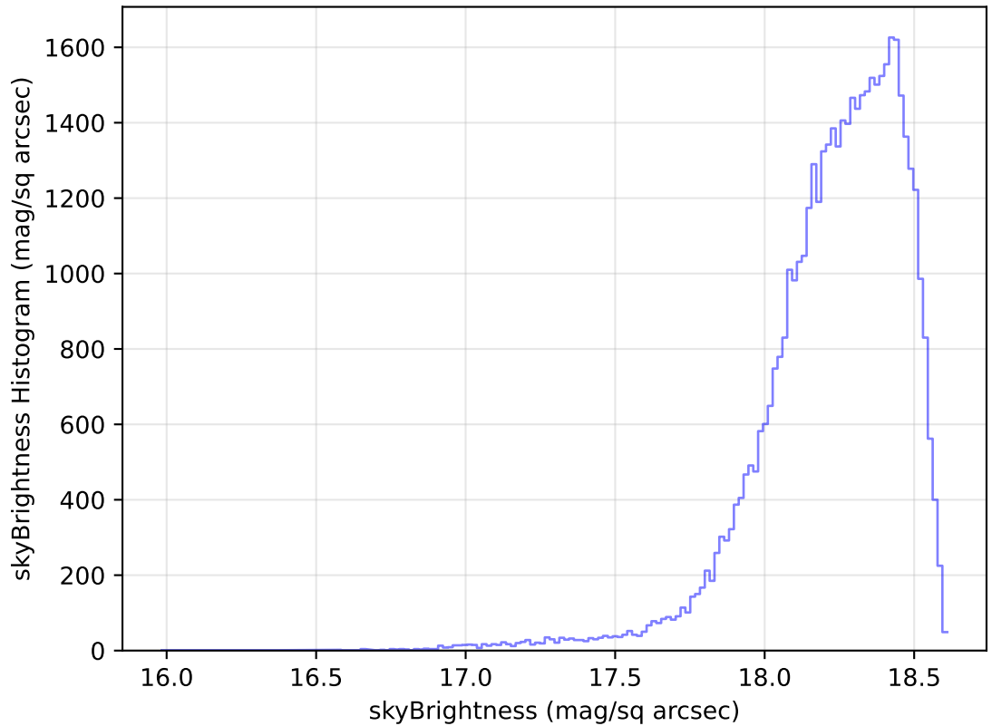
internal_u_expt27_nscale1.2v3.4_10yrs Yr 1 y band: skyBrightness Histogram
