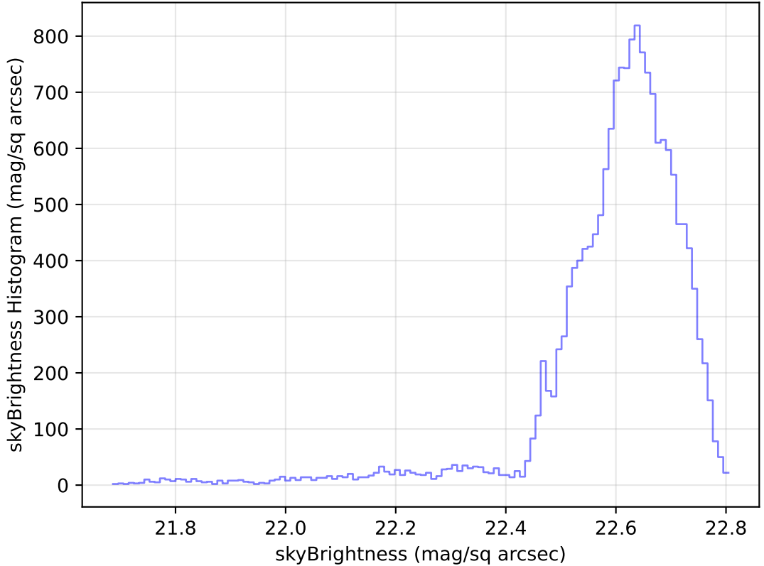
internal_u_expt27_nscale1.2v3.4_10yrs Yr 1 u band: skyBrightness Histogram
