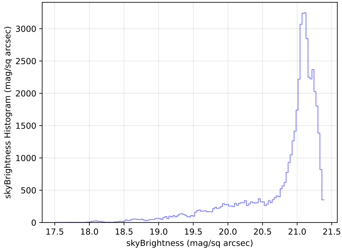
internal_u_expt27_nscale1.2v3.4_10yrs Yr 1 r band: skyBrightness Histogram
