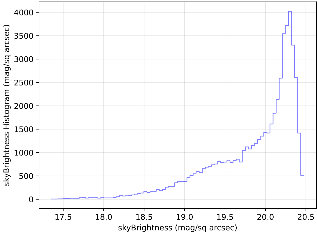
internal_u_expt27_nscale1.2v3.4_10yrs Yr 1 i band: skyBrightness Histogram
