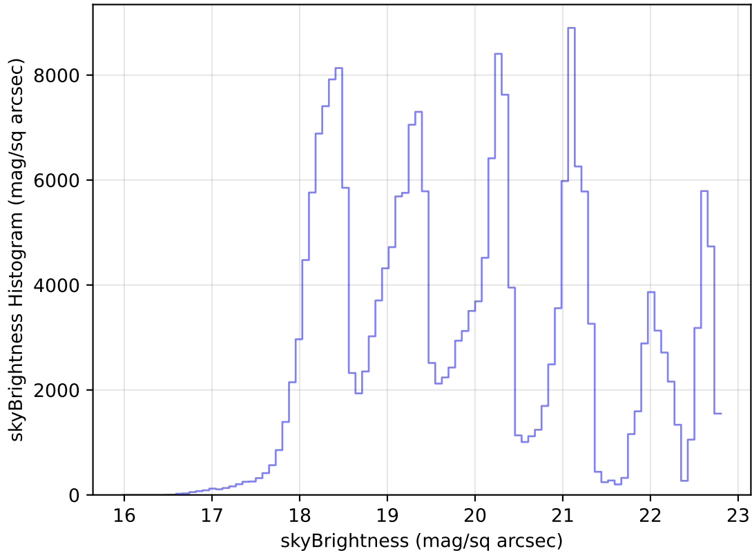
internal_u_expt27_nscale1.2v3.4_10yrs Yr 1 all bands: skyBrightness Histogram
