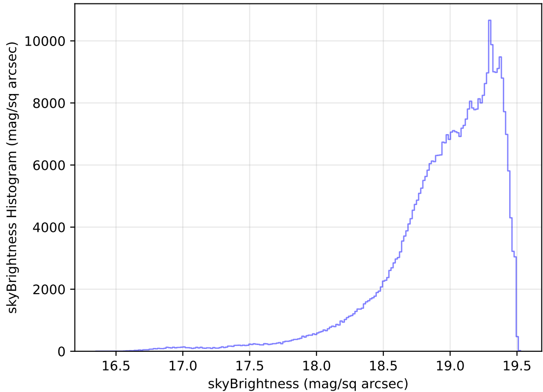
internal_u_expt27_nscale1.2v3.4_10yrs WFD z band: skyBrightness Histogram
