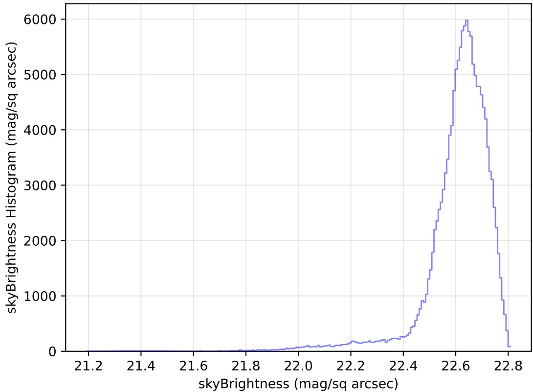
internal_u_expt27_nscale1.2v3.4_10yrs WFD u band: skyBrightness Histogram
