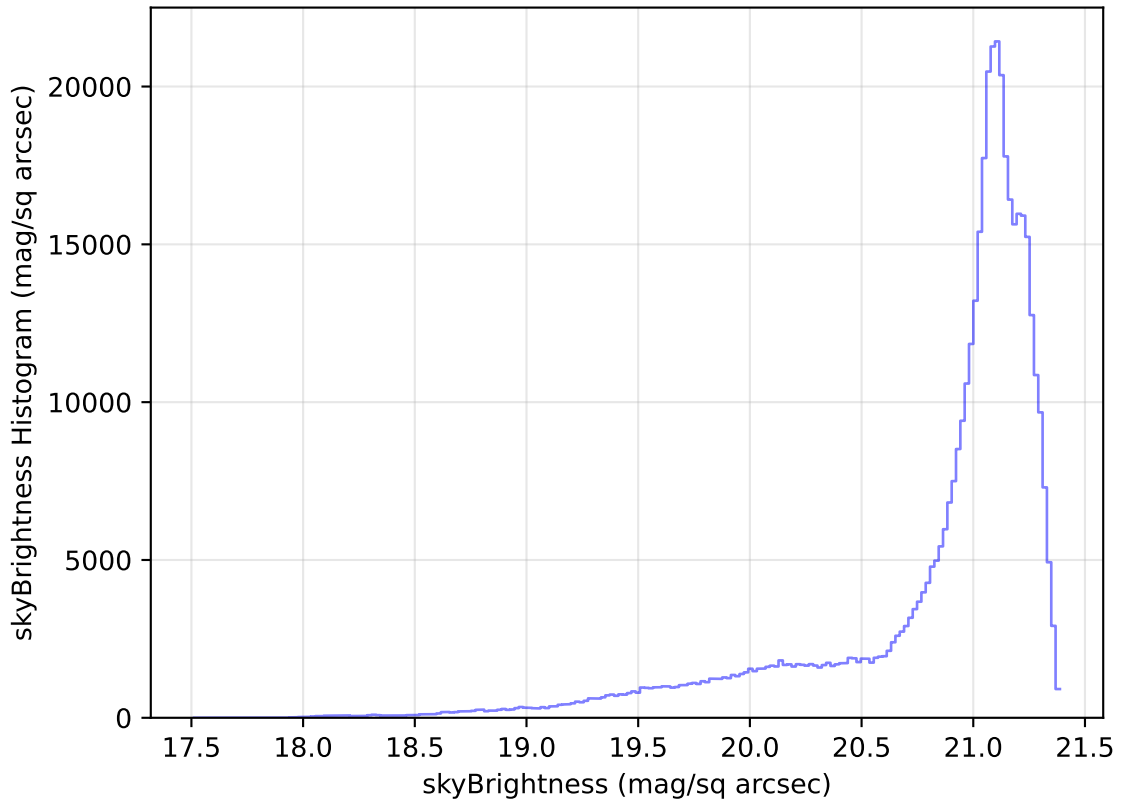
internal_u_expt27_nscale1.2v3.4_10yrs WFD r band: skyBrightness Histogram
