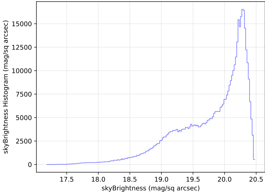
internal_u_expt27_nscale1.2v3.4_10yrs WFD i band: skyBrightness Histogram
