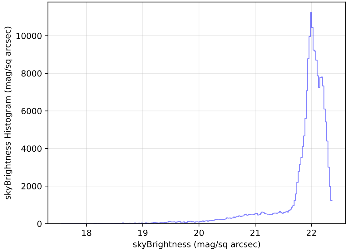
internal_u_expt27_nscale1.2v3.4_10yrs WFD g band: skyBrightness Histogram
