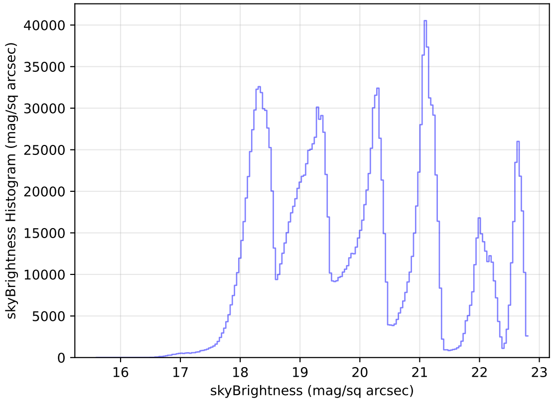
internal_u_expt27_nscale1.2v3.4_10yrs WFD all bands: skyBrightness Histogram
