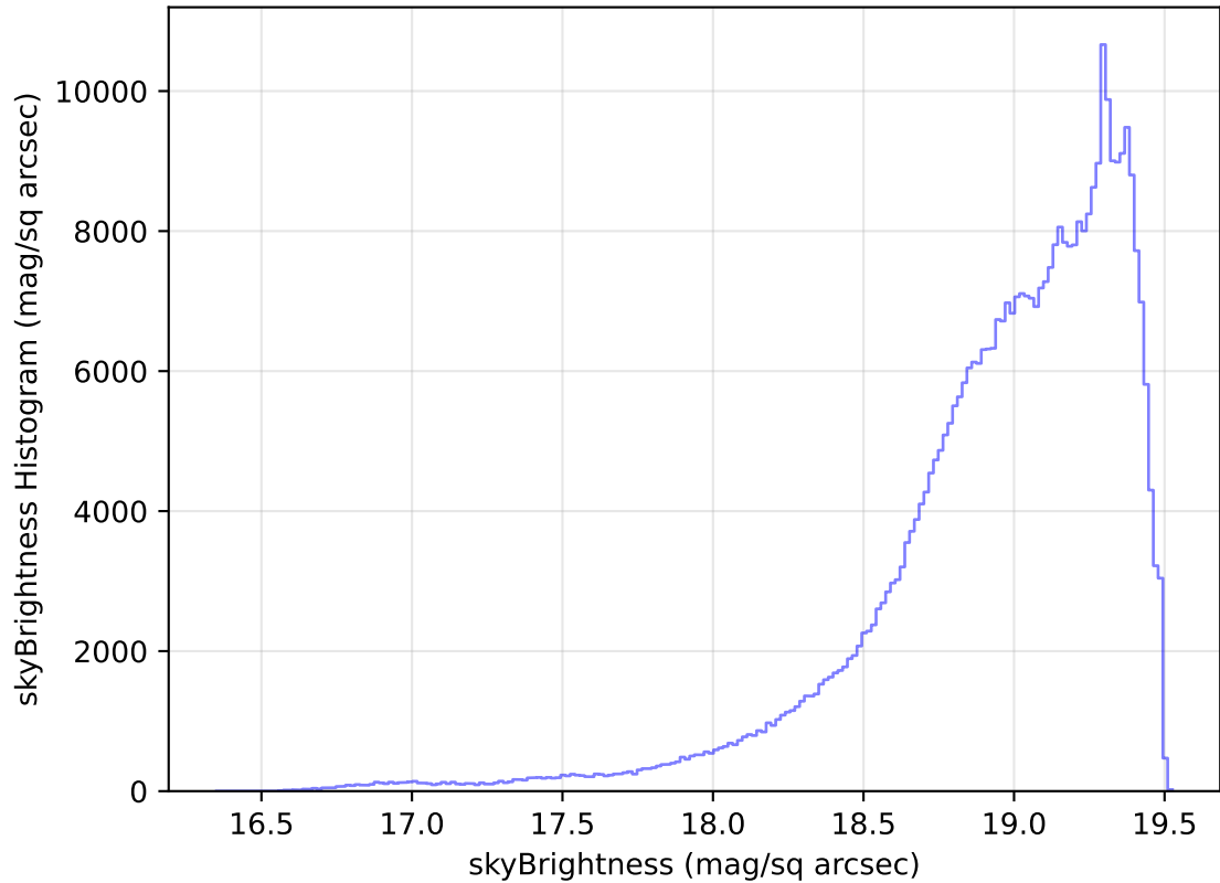
internal_u_expt27_nscale1.2v3.4_10yrs All sky z band: skyBrightness Histogram
