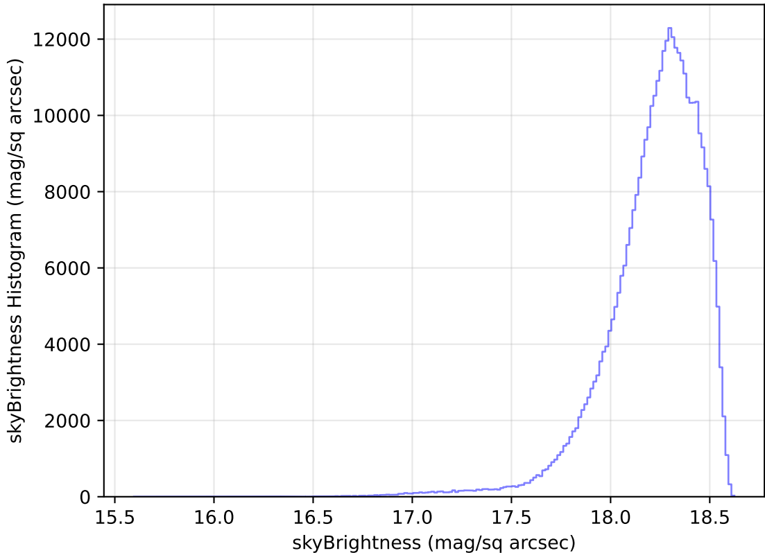
internal_u_expt27_nscale1.2v3.4_10yrs All sky y band: skyBrightness Histogram
