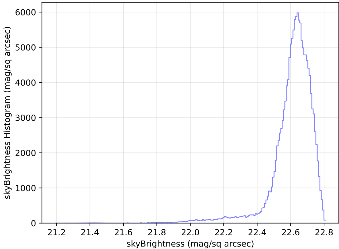
internal_u_expt27_nscale1.2v3.4_10yrs All sky u band: skyBrightness Histogram
