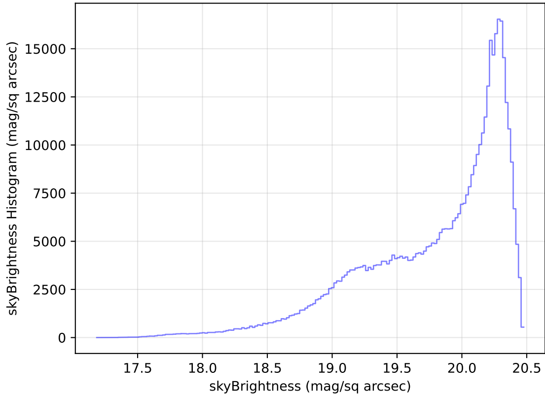
internal_u_expt27_nscale1.2v3.4_10yrs All sky i band: skyBrightness Histogram
