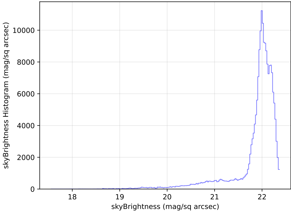
internal_u_expt27_nscale1.2v3.4_10yrs All sky g band: skyBrightness Histogram
