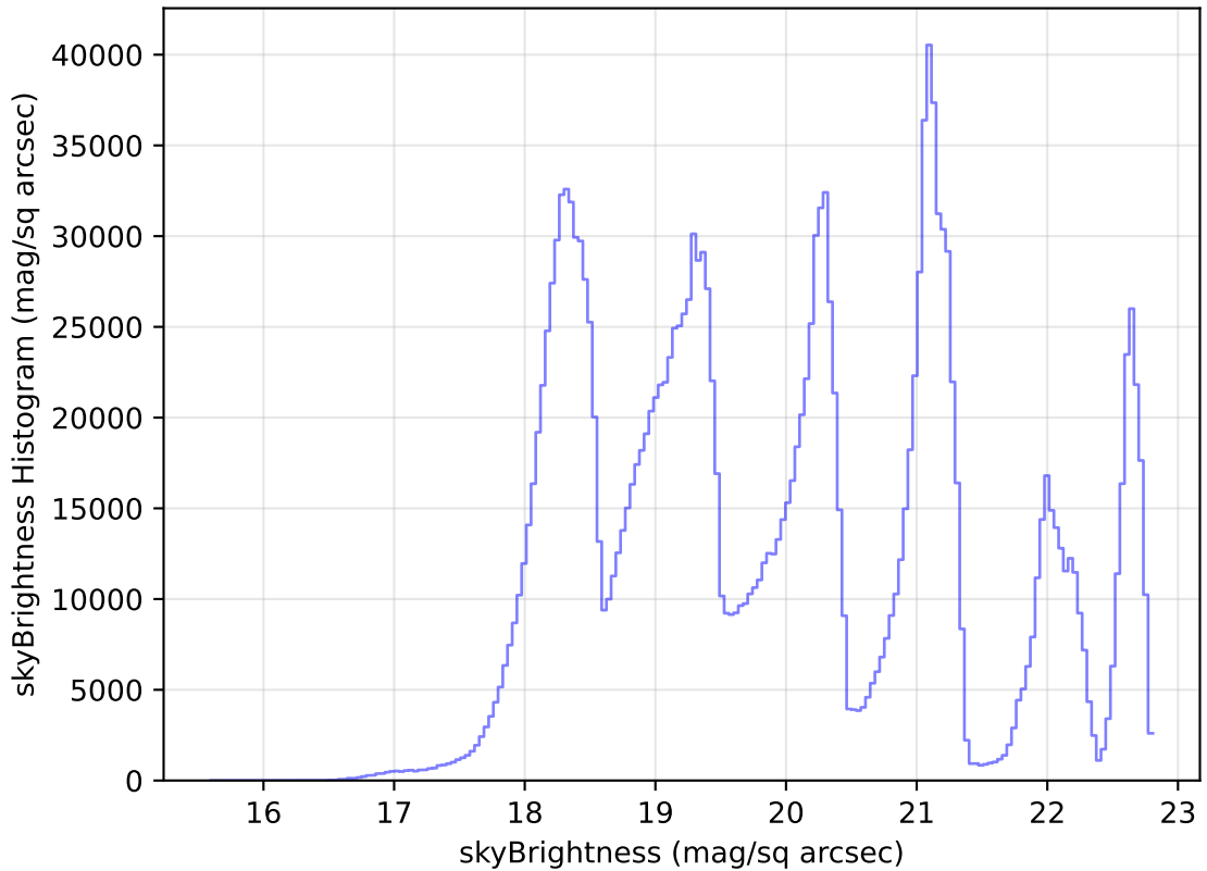
internal_u_expt27_nscale1.2v3.4_10yrs All sky all bands: skyBrightness Histogram
